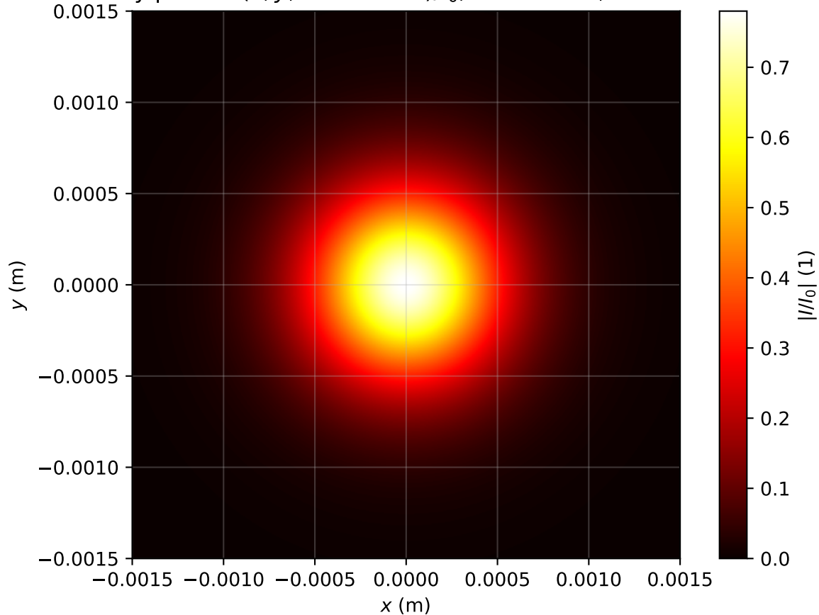
Intensity profile I(x, y, z = 2.149m)/I_0 , Pin=0.5Pcr, artificial time
